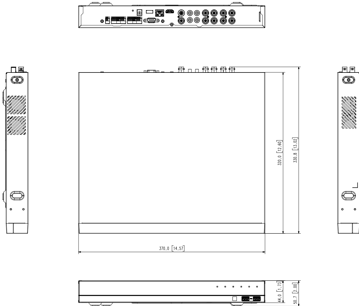
Appearance drawing HRX-820 Unit : mm[inches]
